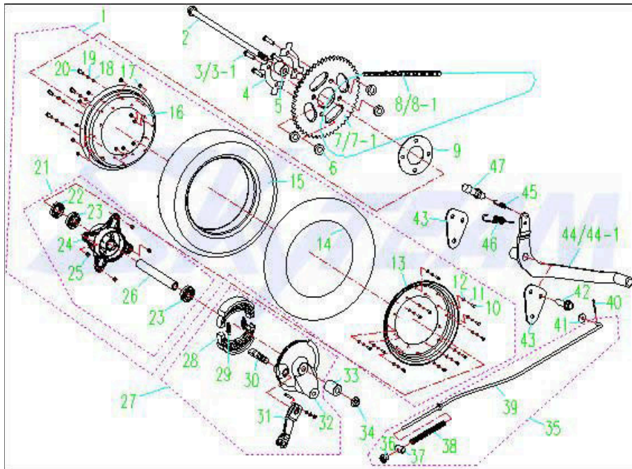
Fig. 11 REAR WHEEL
